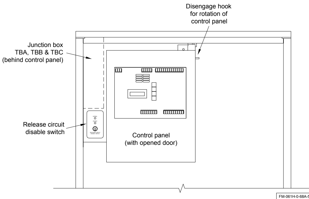
Figure 4.3 - PFC-4410RC control panel detail
