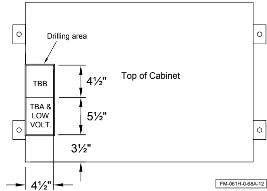
Figure 6.1 - Drilling details
