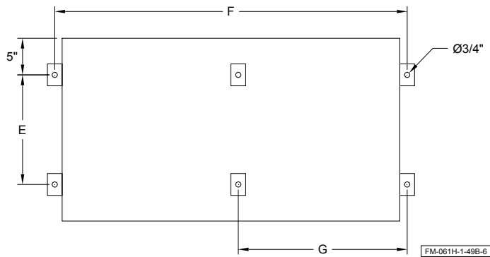
Figure 6.3 - Floor anchoring template
