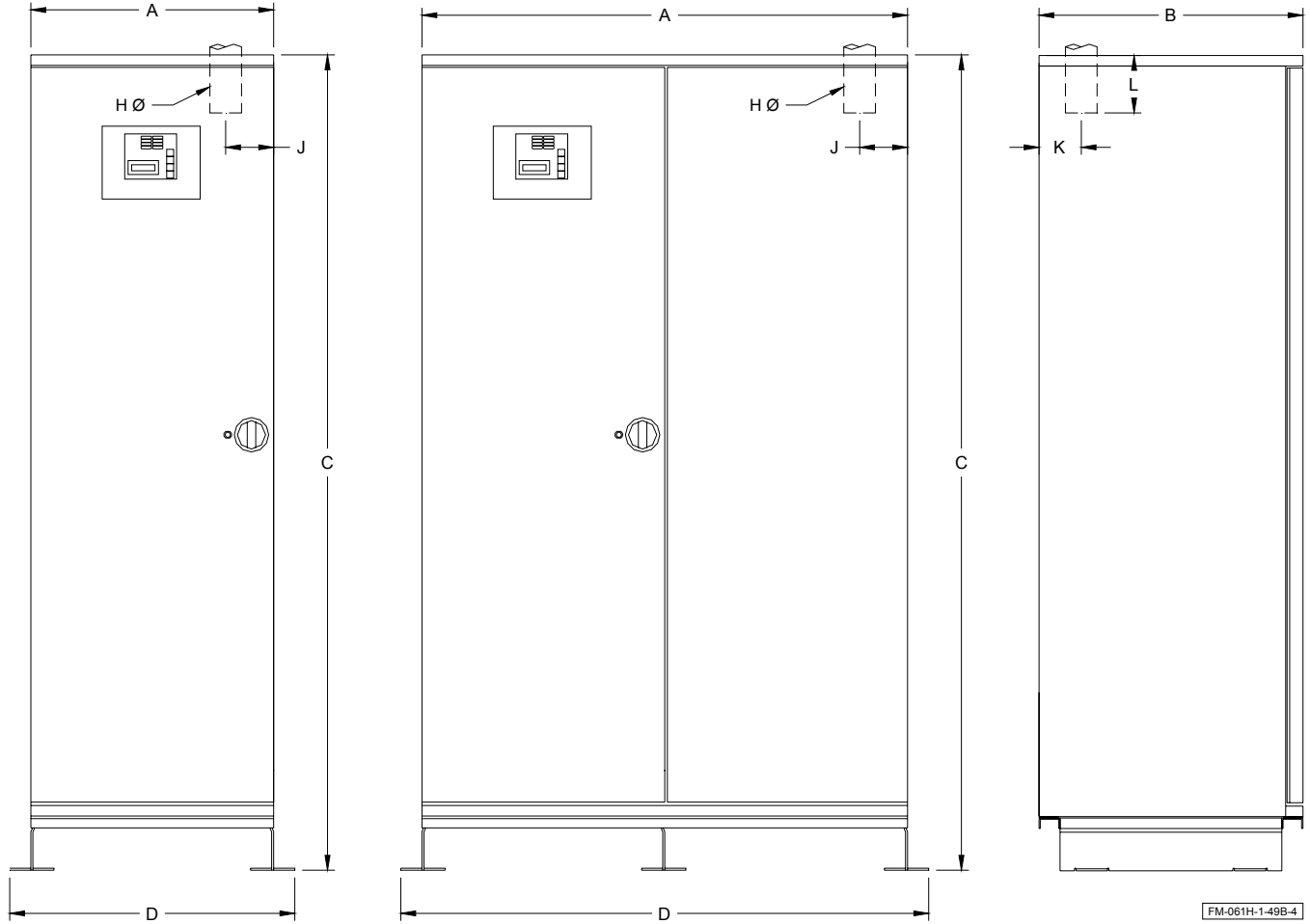
Figure 6.2 - Cabinet dimensions
