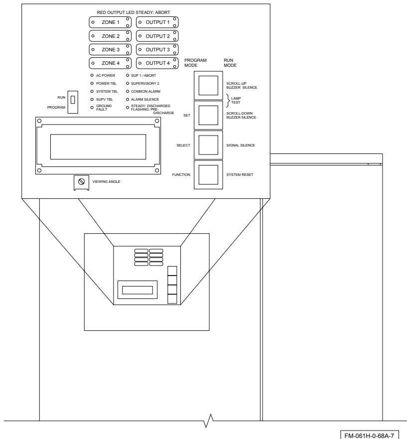
Figure 4.3 - PFC-4410RC control panel detail
