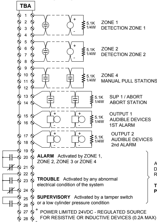
Figure 5.1 - Field wiring diagrams
