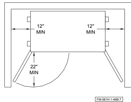
Figure 6.4 - Required clearance
